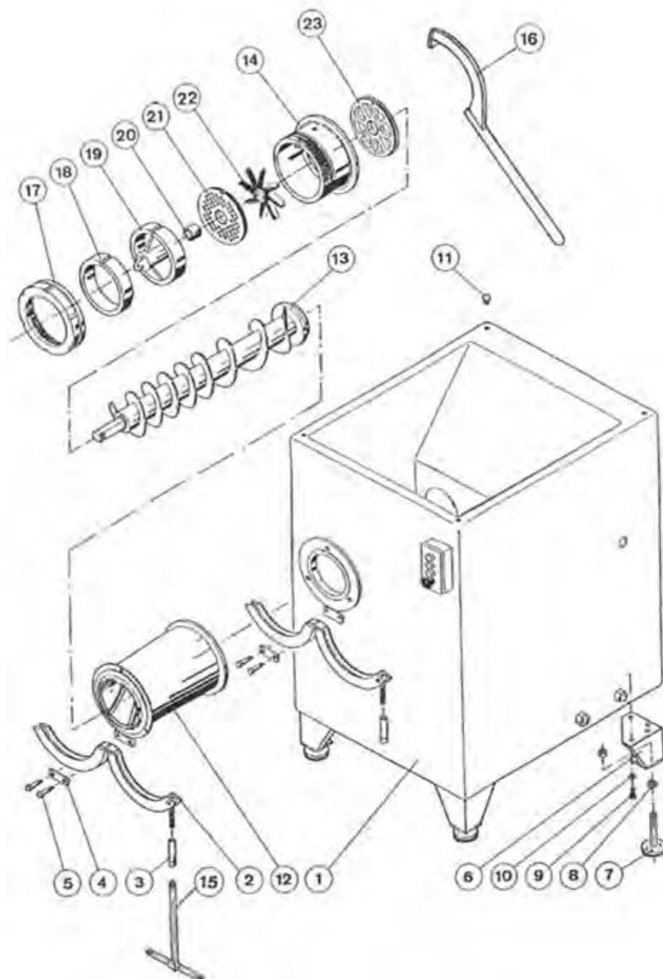
Exploded View of Wolfking® Grinder C.250/300-UNI
